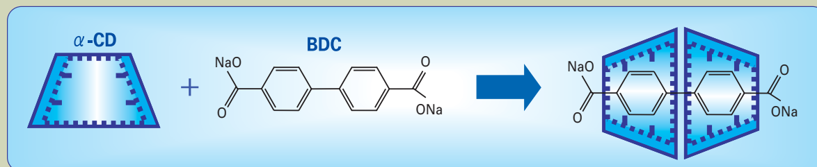
Fig. 16 Formation of the BDC and \alpha CD dimer inclusion complex.
